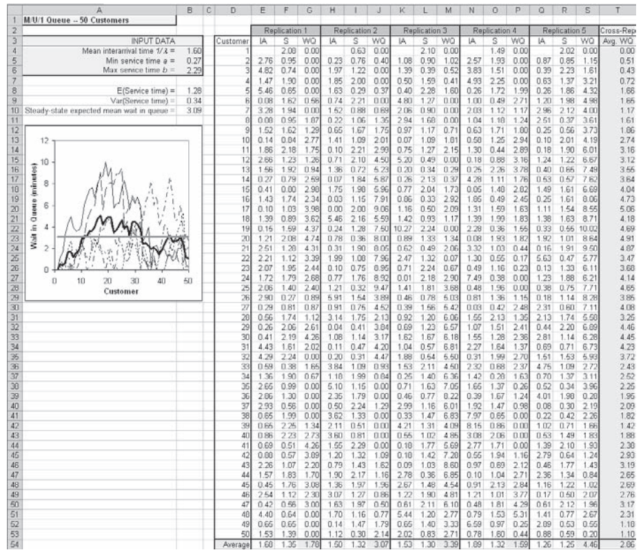
Figure 2-6. Spreadsheet Simulation of the M/U/1 Queue
