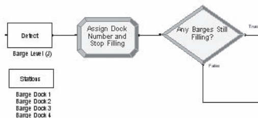
Figure 11-7. Detect Logic for Full Barges
