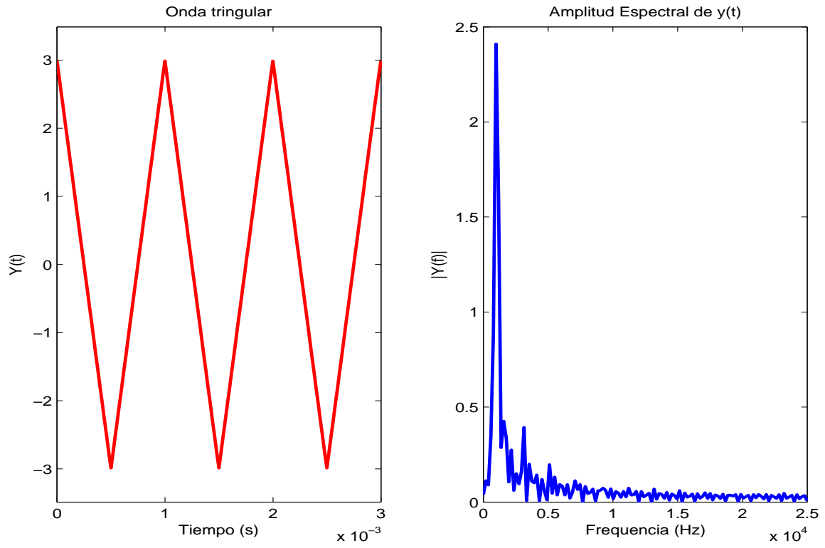
Figure 5: Onda triangular.
